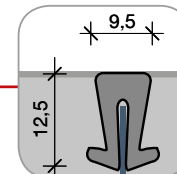
pvc profiel 3 permanent
